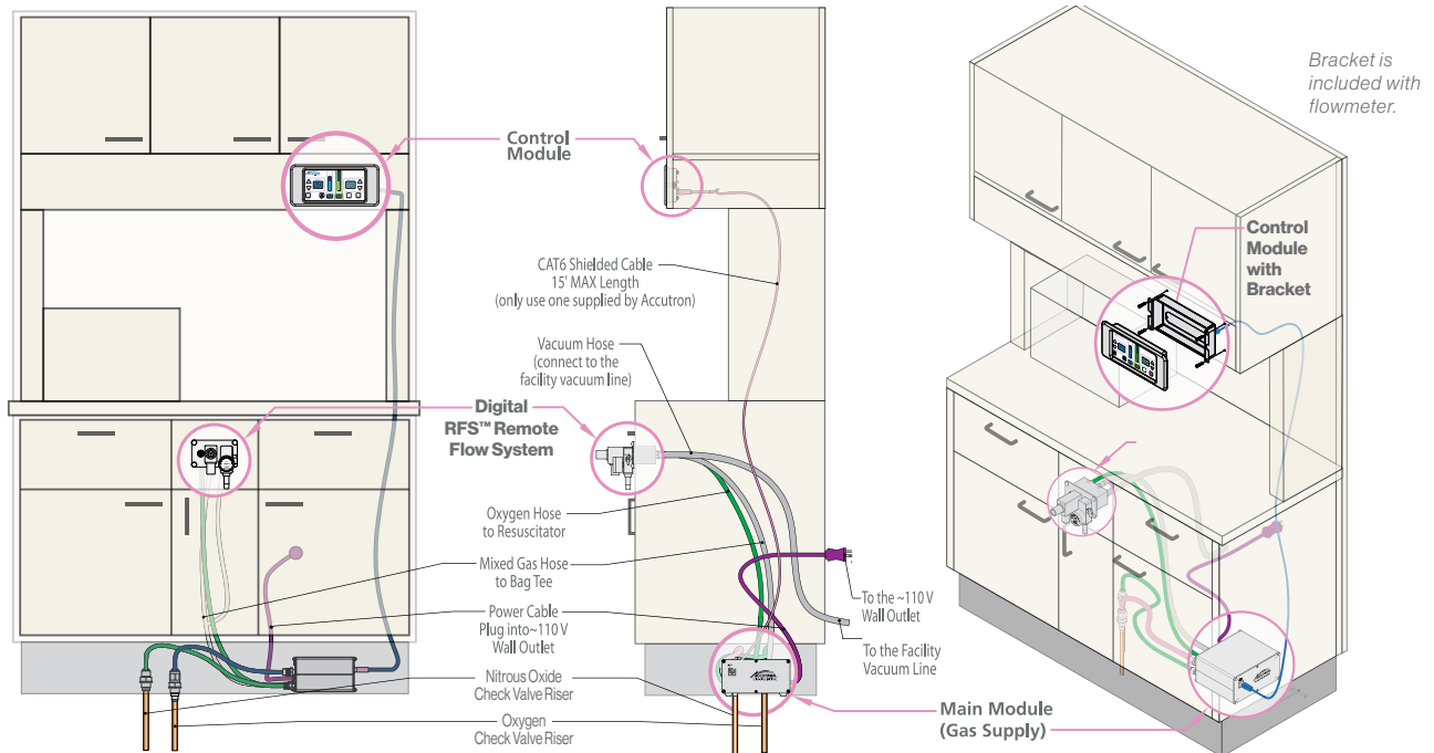
In-cabinet illustrations are specific to 56800 Digital Ultra™ Flushmount with RFS™ Remote Flow System Vacuum Controller.
